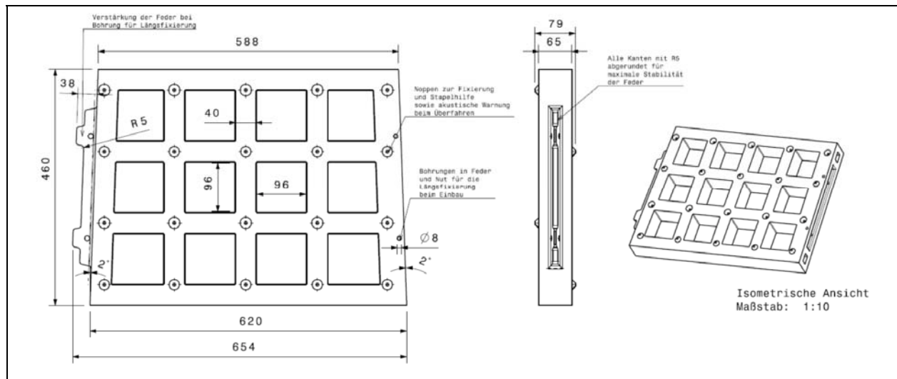
Trapezoid honeycomb paver 650 x 460 x 65mm, single angle 2°, installation circular 4°
